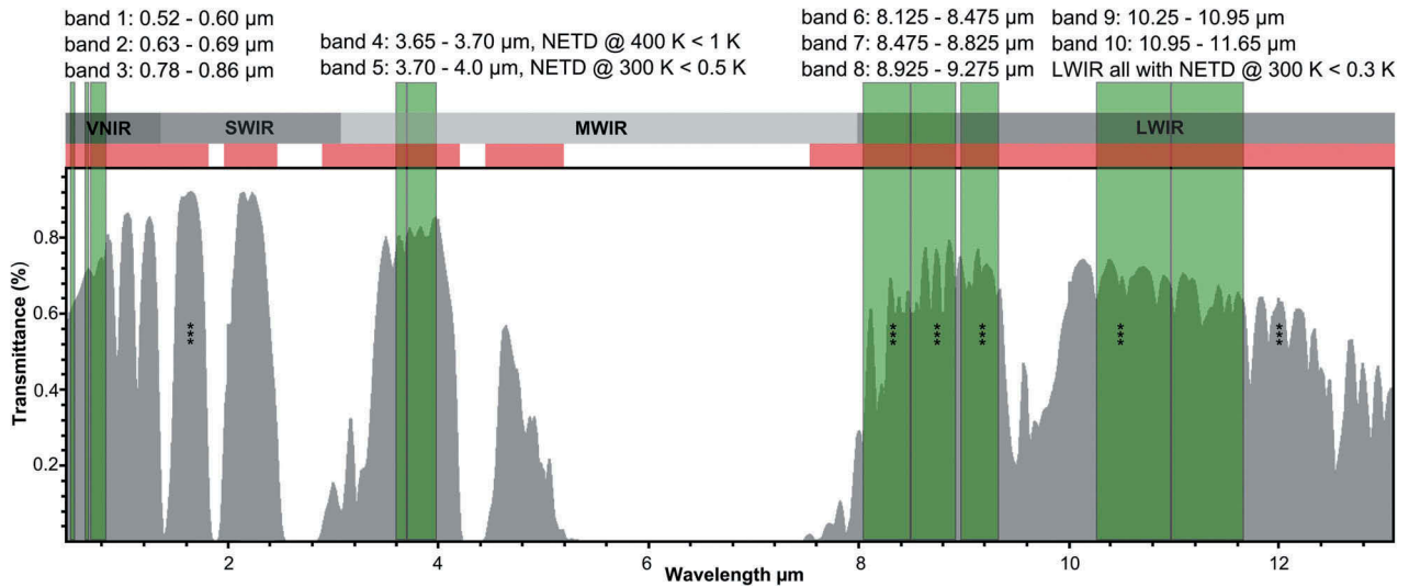
Figure 1. Atmospheric transmittance and DIEGO's spectral bands specification in comparison with ECOSTRESS's spectral bands marked with ***. DIEGO's spectral band 11 (not shown) can be used to enhance atmospheric correction or for CO 2 detection, but it is not defined yet. Transmittance is calculated with modtran ( http://modtran.spectral.com/modtran_home ) for mid-latitude summer, top of atmosphere, 294.2 K.
